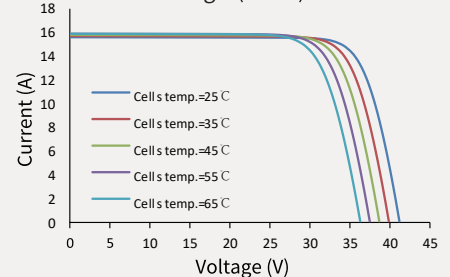
Current-Voltage (520W)
